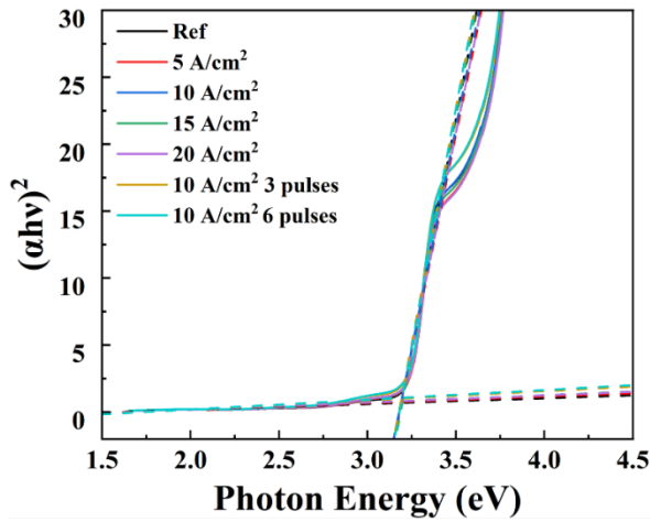
Figure 3 - Tauc plots of ZnO samples
