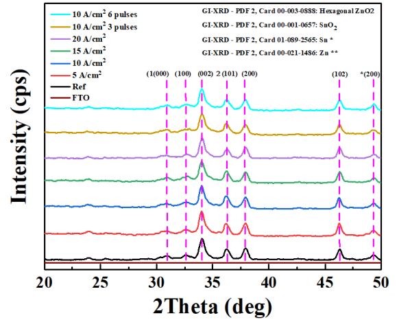
Figure 4 - GI-XRD patterns of ZnO samples before and after irradiation
