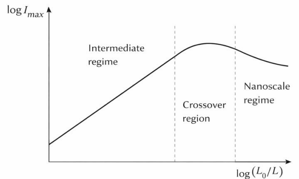
Figure 3. Schematic crossover from apparent exponential scaling of \mathcal{I}_{\max} at intermediate sizes to noise-limited, sub-exponential behavior at the nanoscale.
