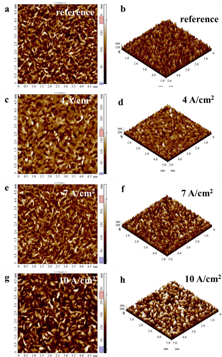
Figure 1 – AFM images of the surface of the CNWs before and after irradiation with an ion beam with different current densities: (a,b) initial sample, (c,d) 4 A/cm 2 , (e,f) 7 A/cm 2 , (g,h) 10 A/cm 2 .
