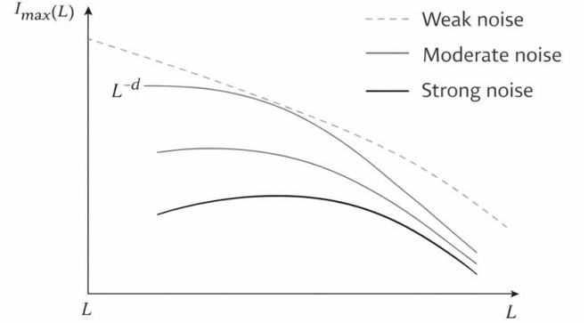
Figure 2. Schematic scaling of the maximum information density \mathcal{I}_{\max}(L) with system size L for different quantum noise strengths, showing noise-induced suppression of the ideal geometric scaling.
